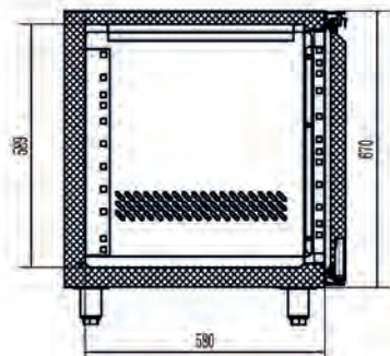
Bokorys GF
